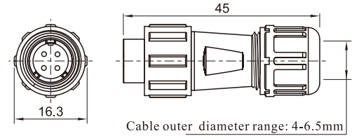
Cable connector Mate with SP1111, SP1112
